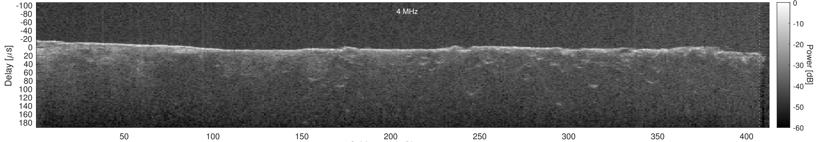
Orbit 15123, Cluttergram
