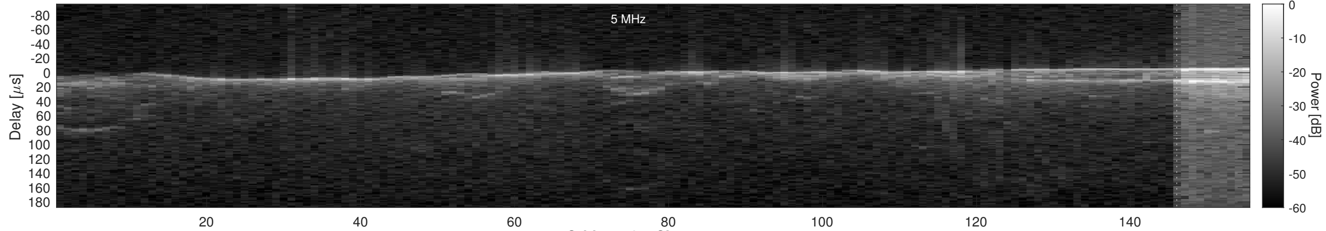
Orbit 15124, Cluttergram
