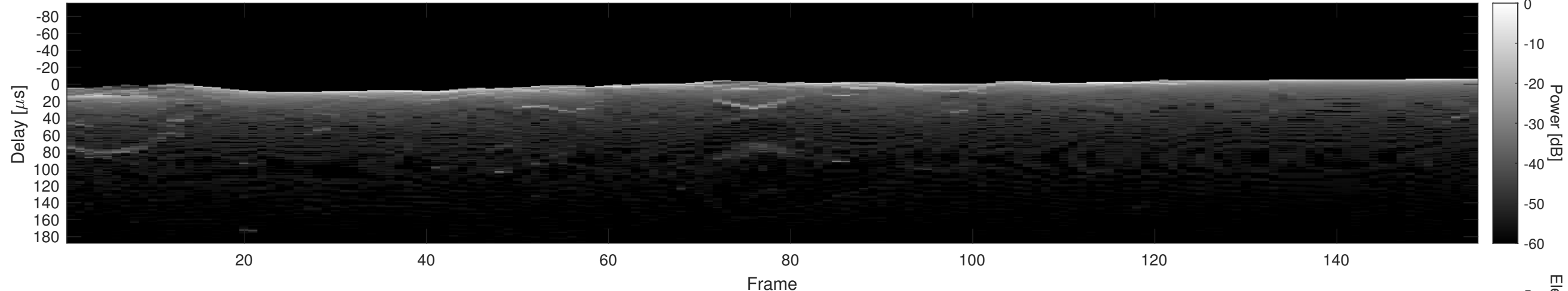
Orbit 15124, Cluttergram
