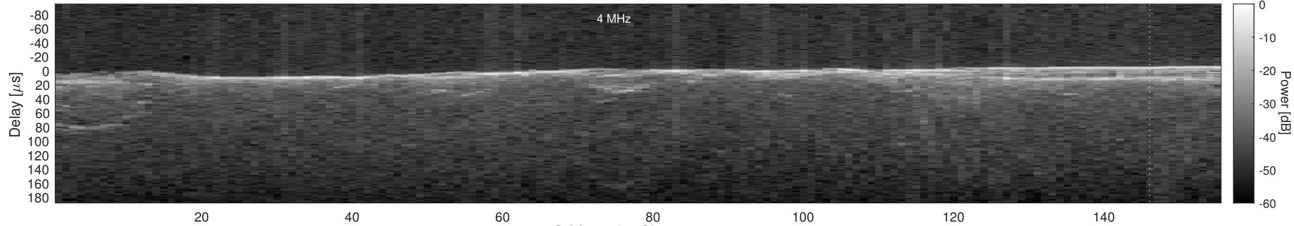
Orbit 15124, Cluttergram
