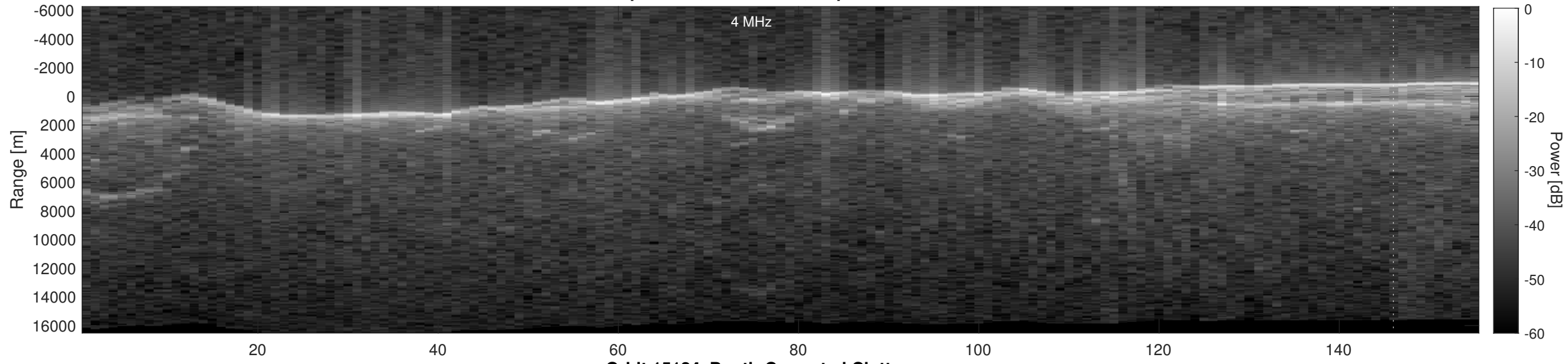
Orbit 15124, Depth-Corrected Cluttergram
