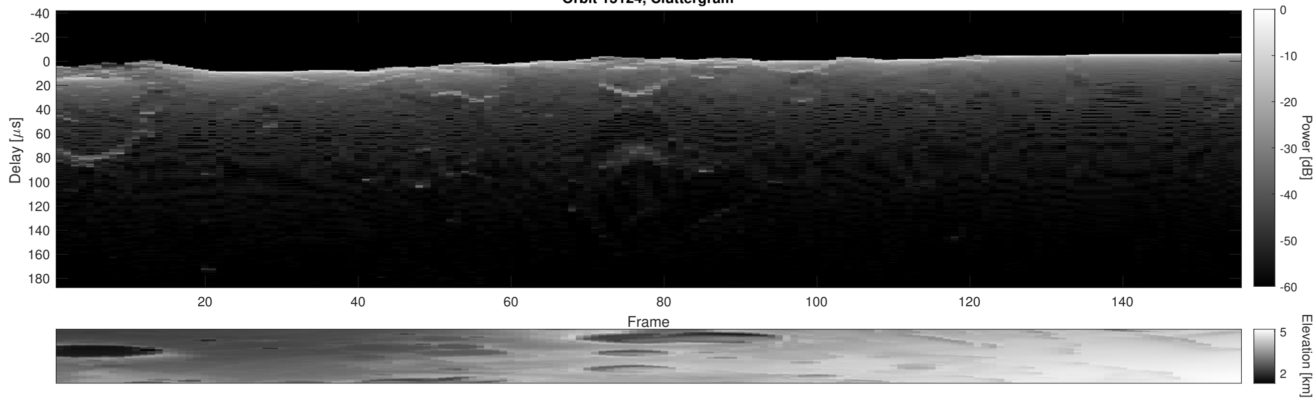
Orbit 15124, Cluttergram
