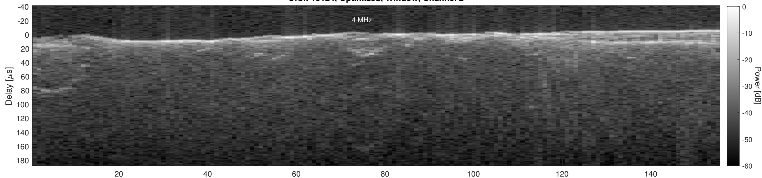
Orbit 15124, Cluttergram
