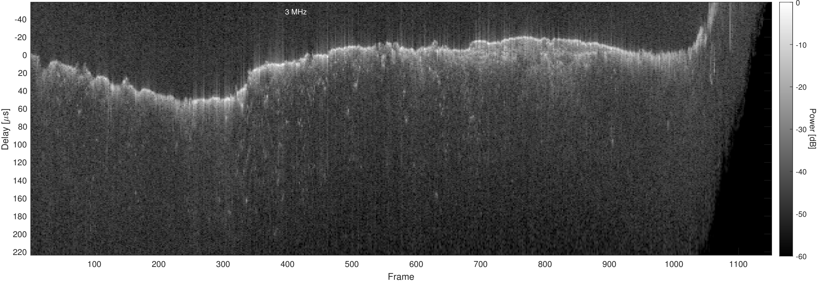
Orbit 15132, Chapman, No Window, Channel 2
