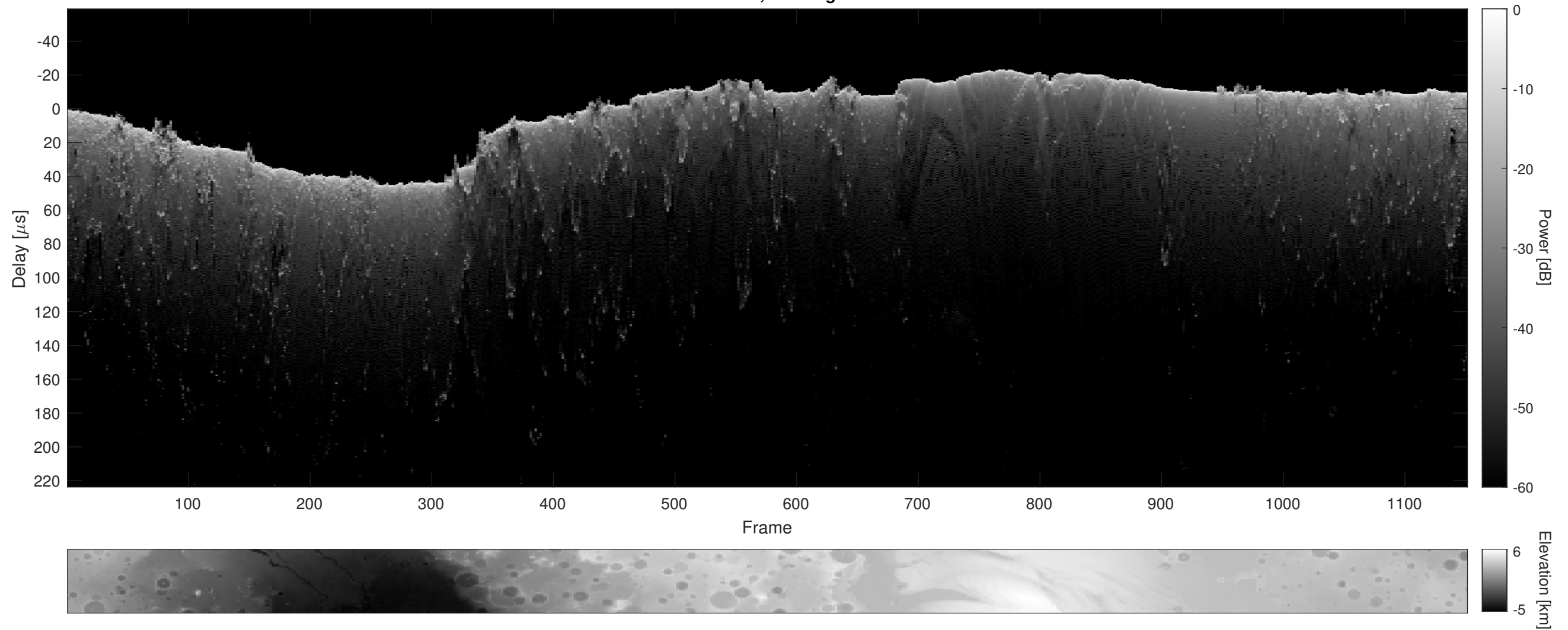
Orbit 15132, Cluttergram
