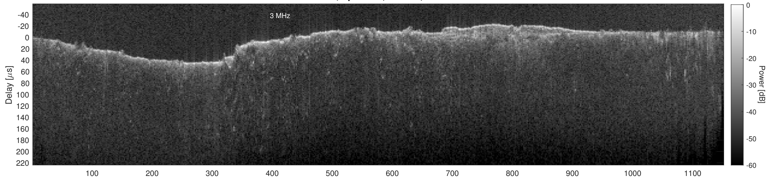
Orbit 15132, Cluttergram
