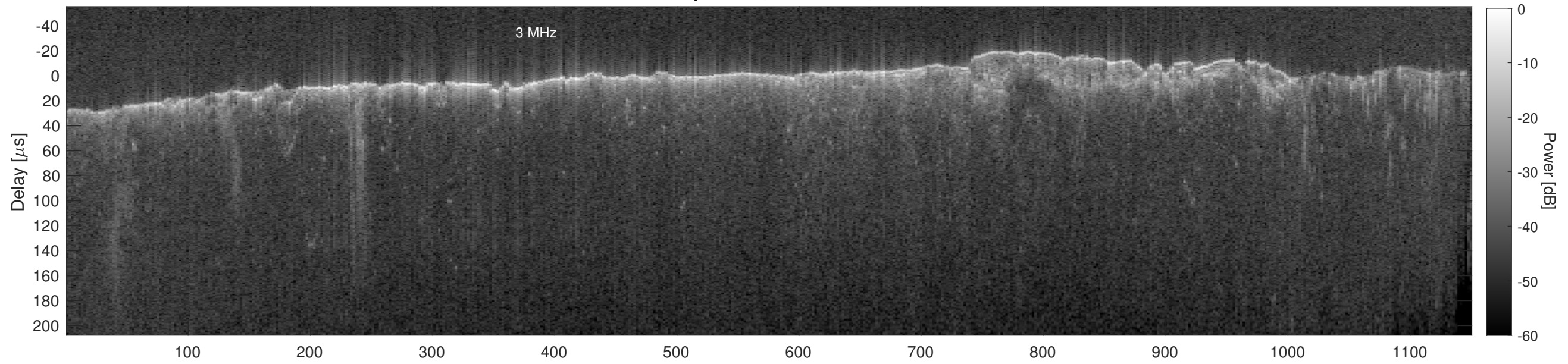
Orbit 15133, Cluttergram
