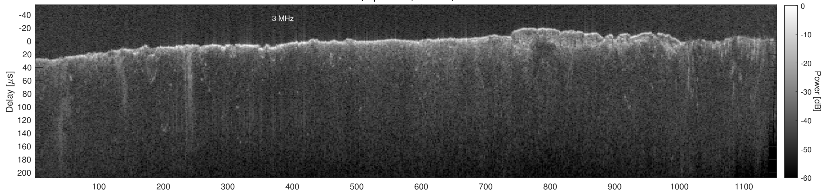
Orbit 15133, Cluttergram
