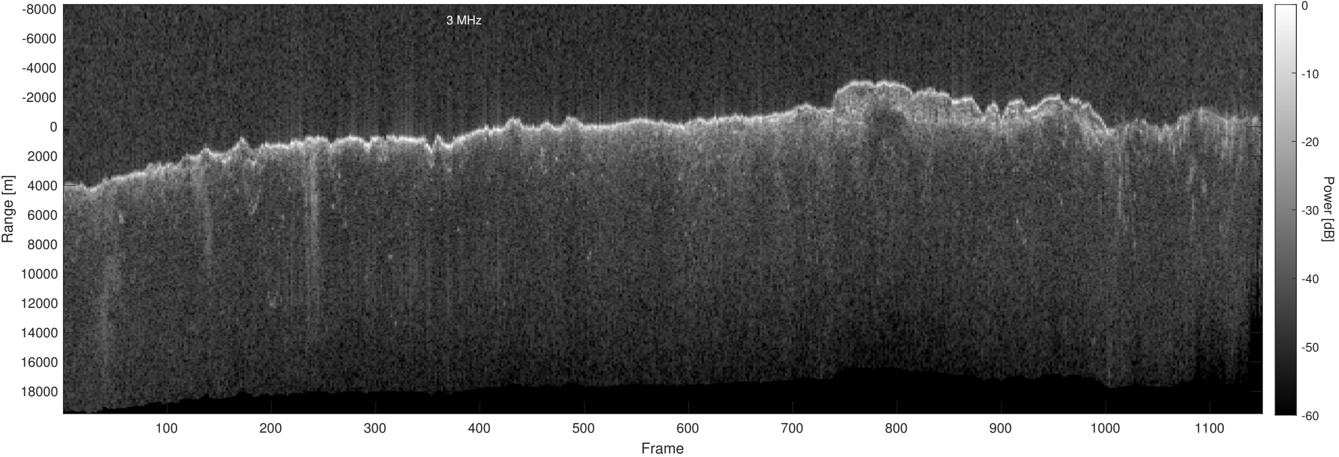
Orbit 15133, Optimized, Window, Depth-Corrected, Channel 2
