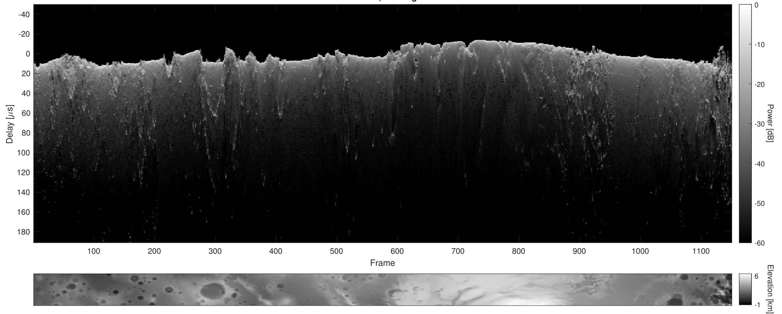
Orbit 15135, Cluttergram
