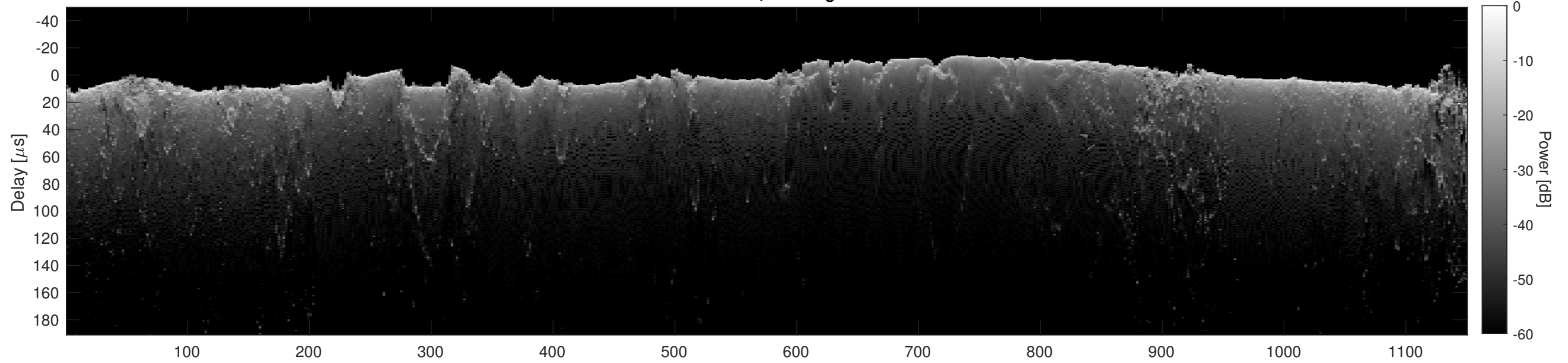
Orbit 15135, Cluttergram
