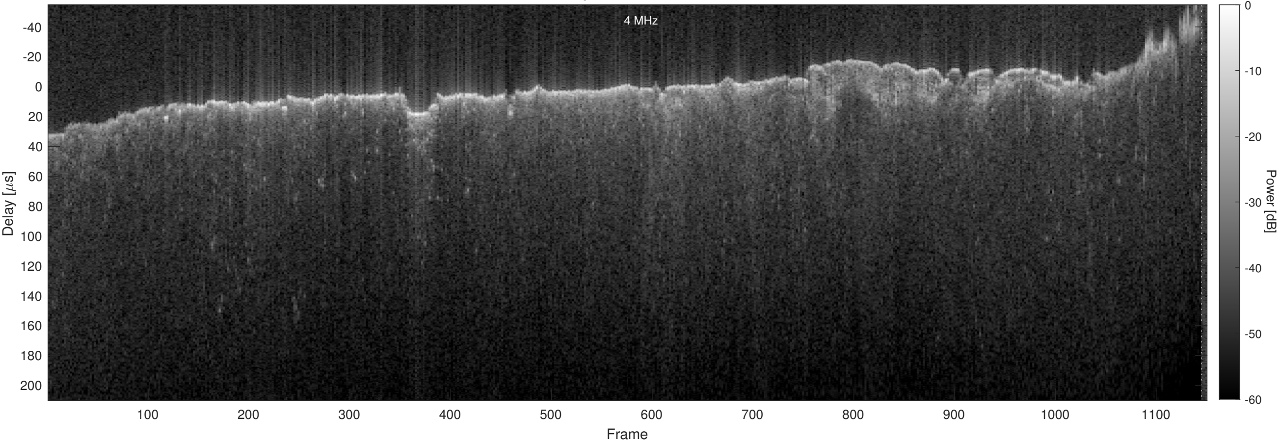
Orbit 15140, Chapman, No Window, Channel 2
