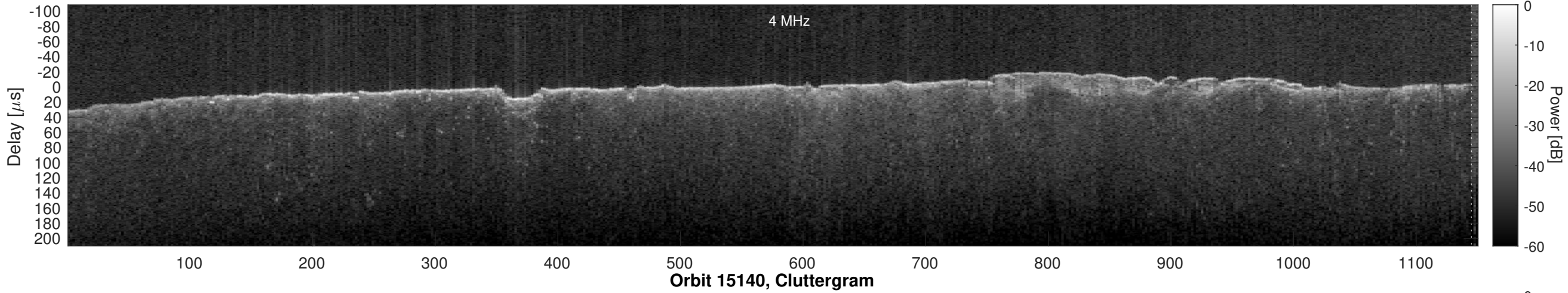
Orbit 15140, Window, Channel 1, Optimized
