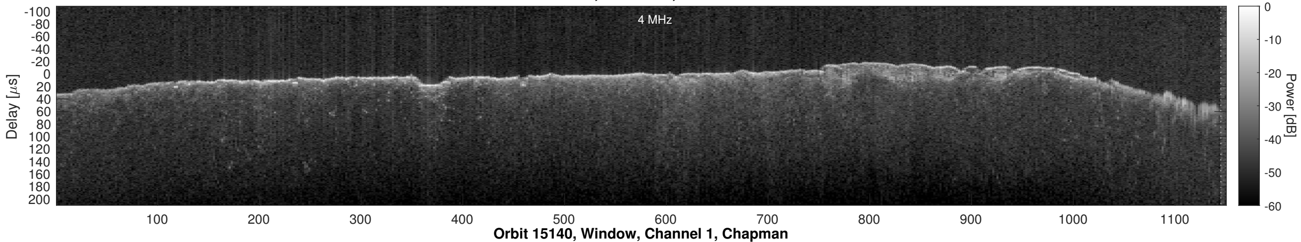
Orbit 15140, Channel 1, Uncorrected
