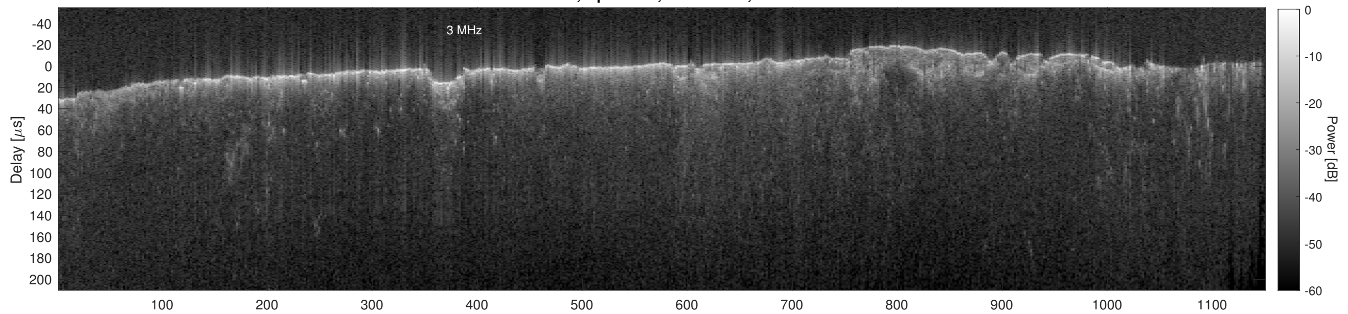
Orbit 15140, Cluttergram
