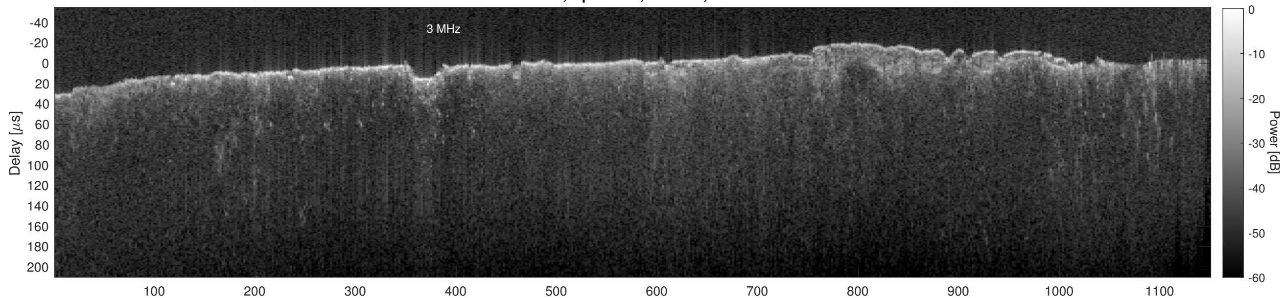
Orbit 15140, Cluttergram
