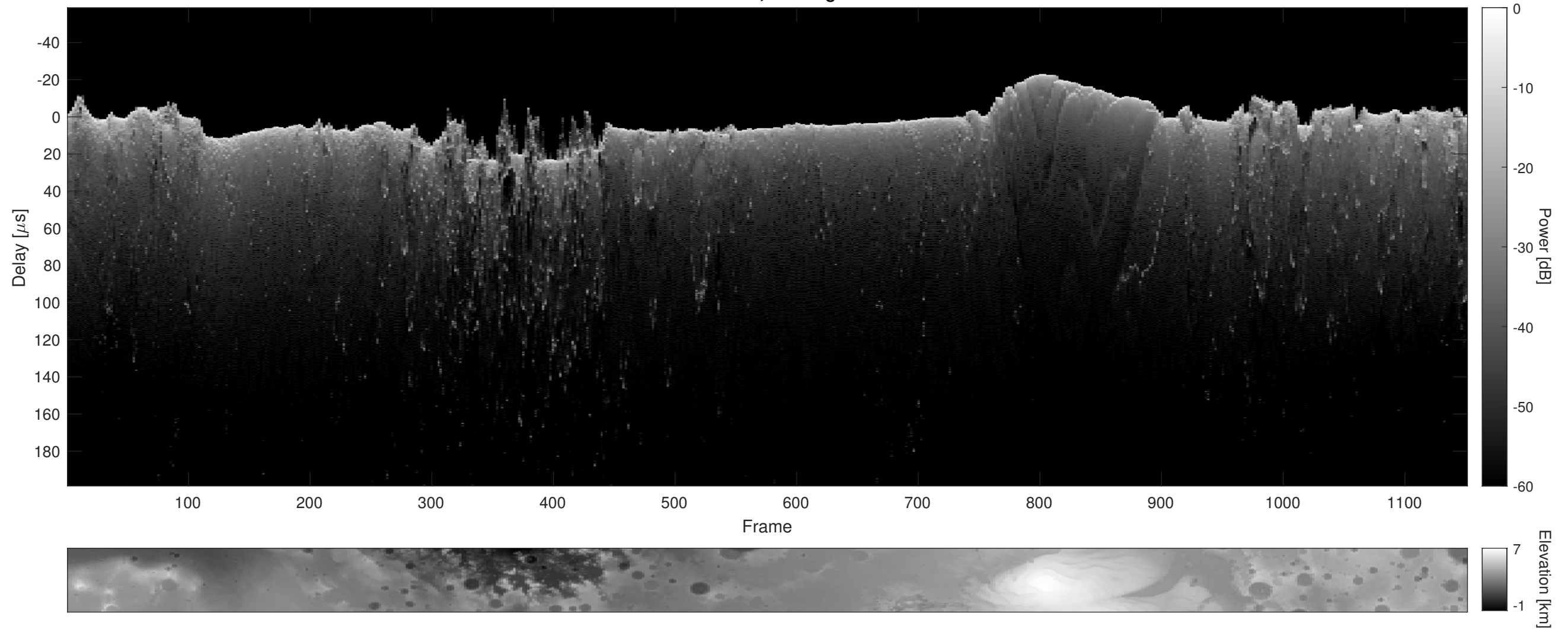
Orbit 15144, Cluttergram
