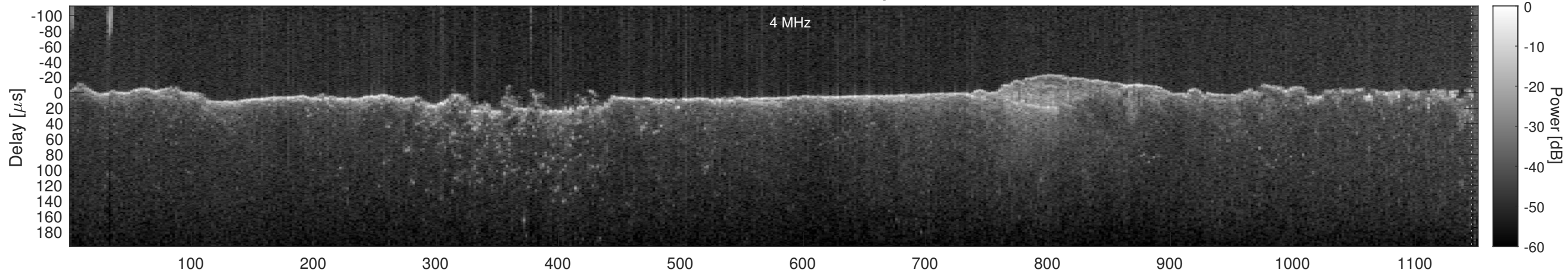
Orbit 15144, Cluttergram
