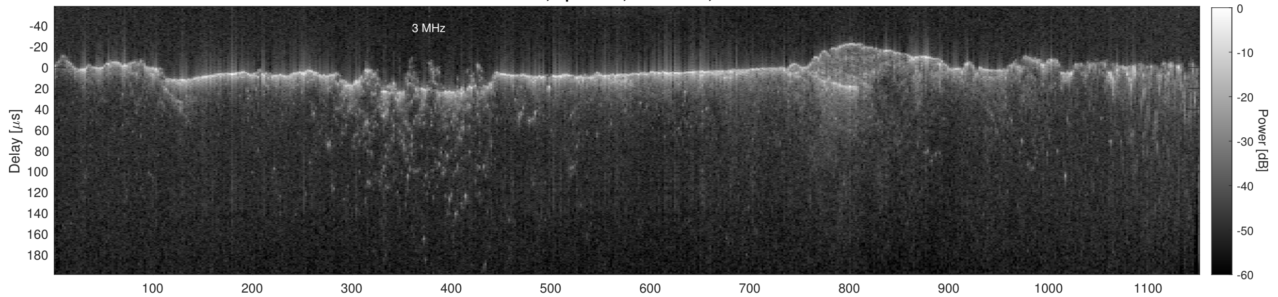
Orbit 15144, Cluttergram
