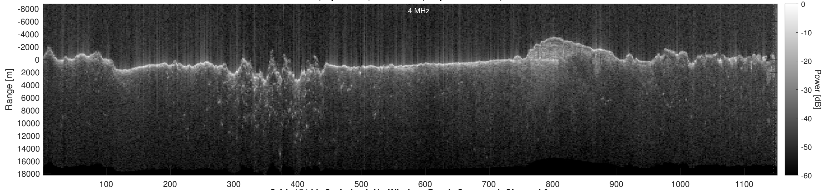
Orbit 15144, Optimized, No Window, Depth-Corrected, Channel 2
