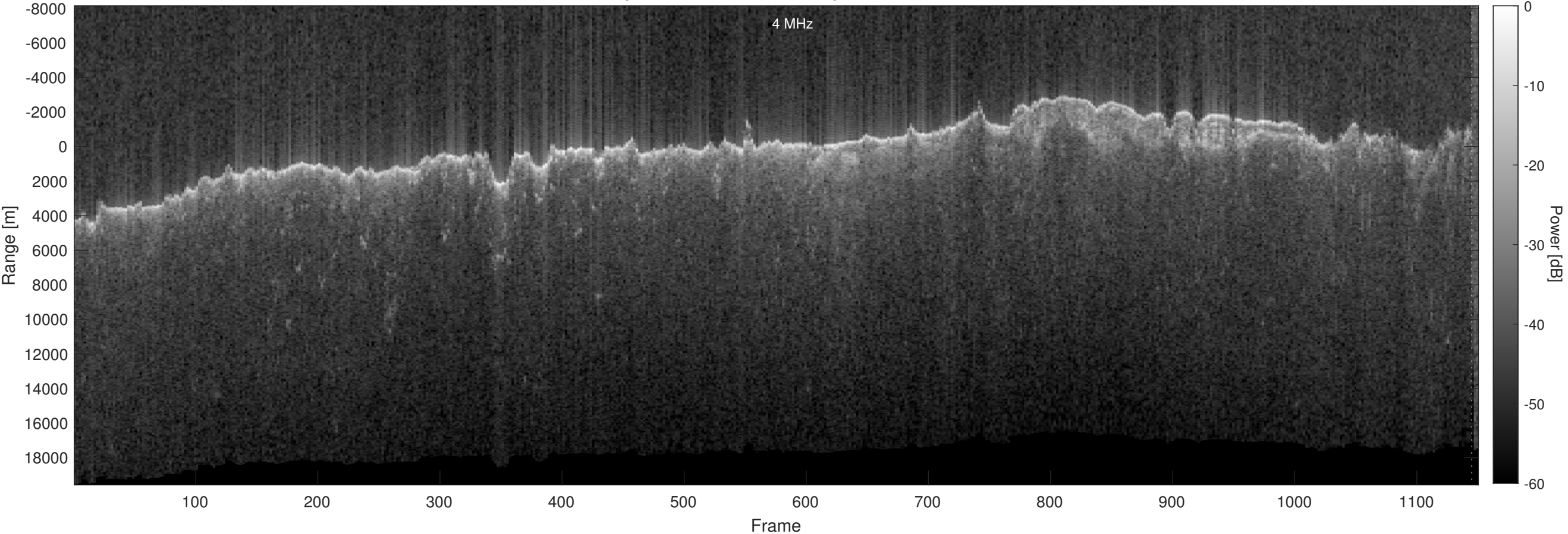
Orbit 15147, Optimized, No Window, Depth-Corrected, Channel 2
