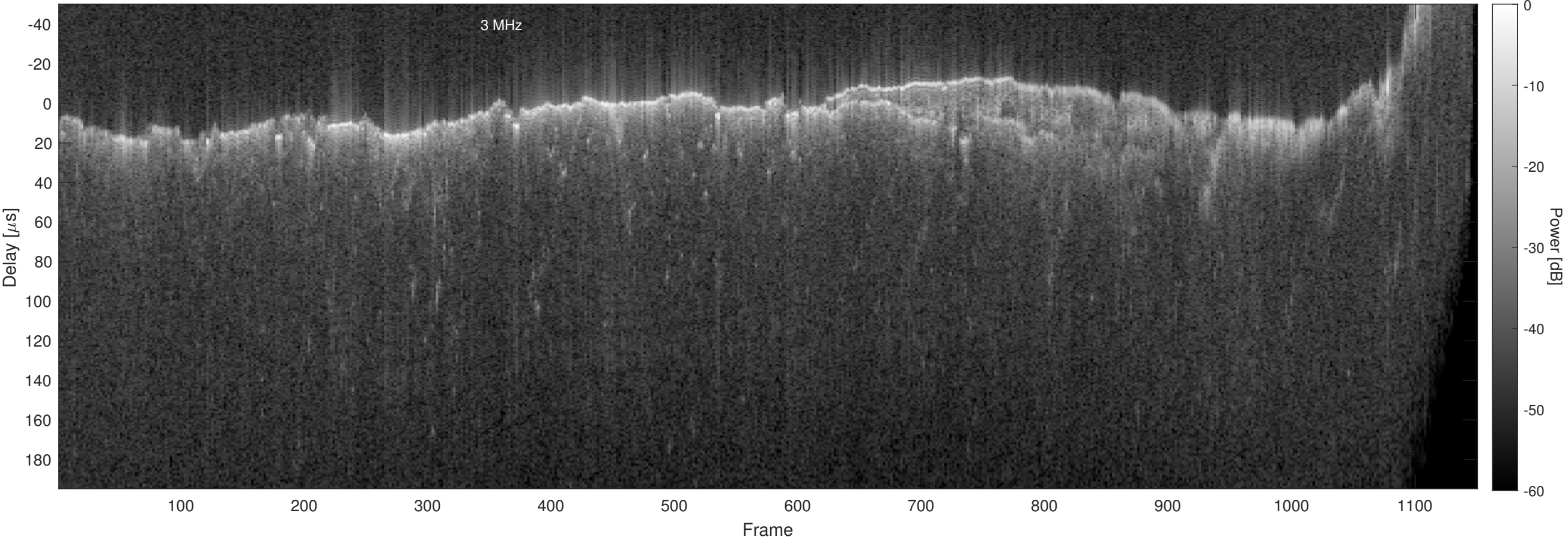
Orbit 15149, Chapman, No Window, Channel 2
