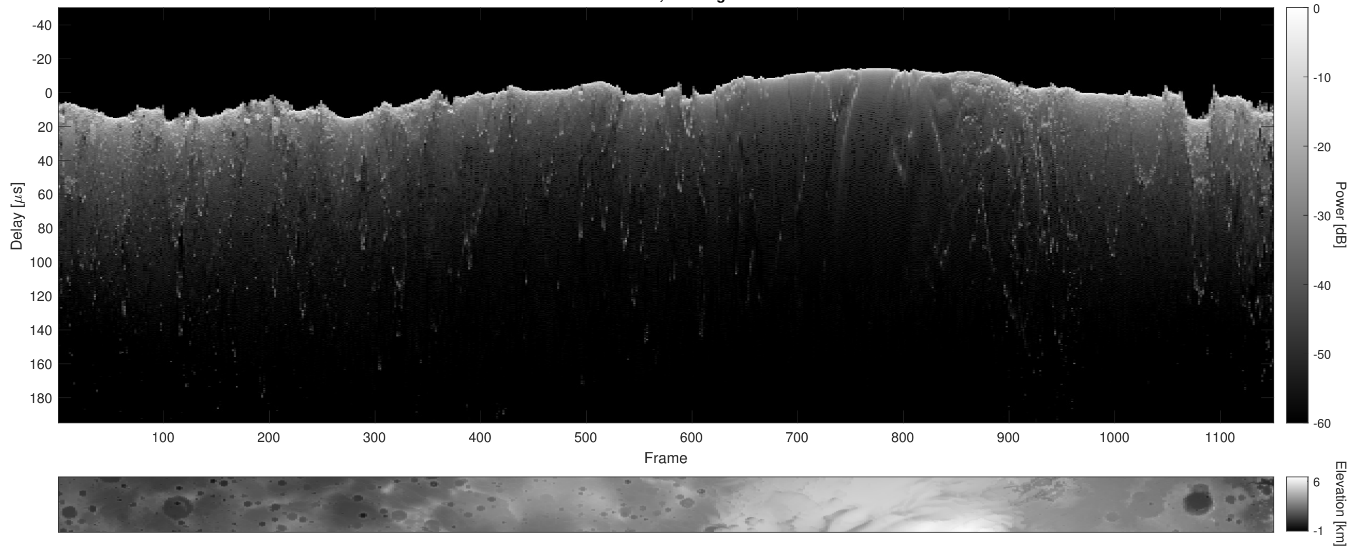
Orbit 15149, Cluttergram
