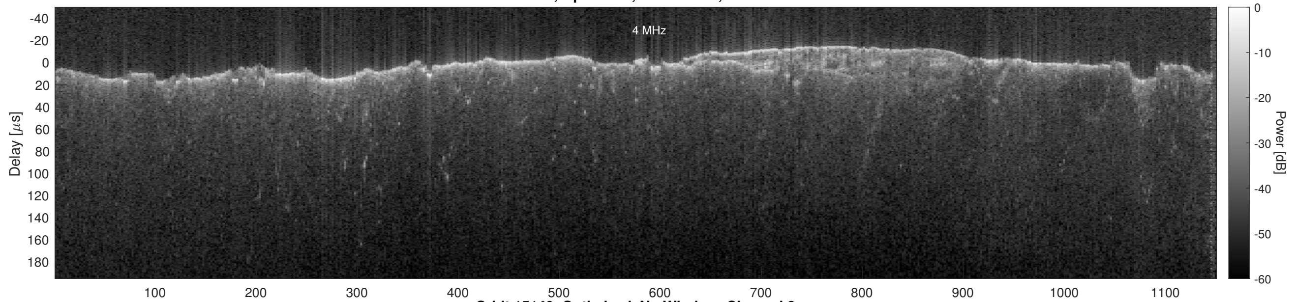
Orbit 15149, Optimized, No Window, Channel 2
