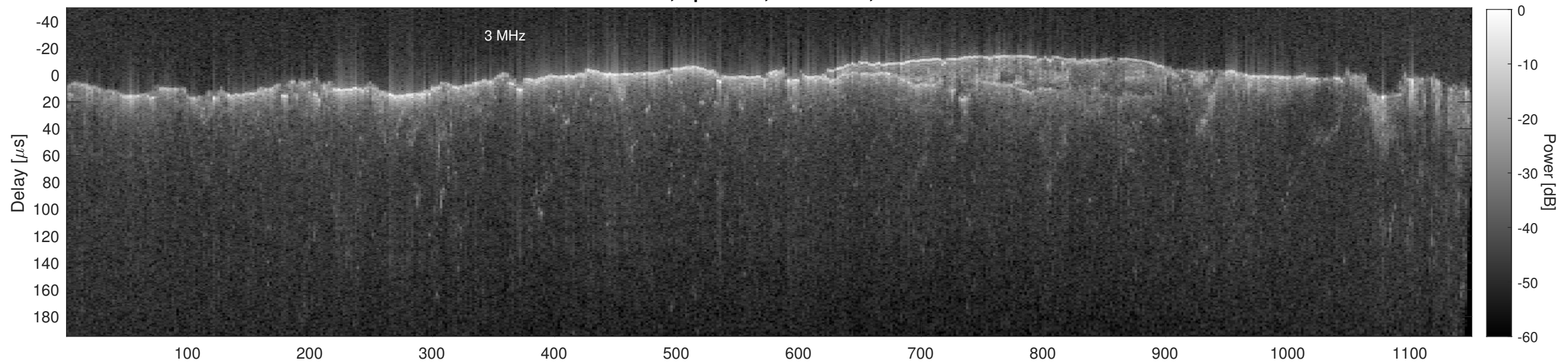
Orbit 15149, Cluttergram
