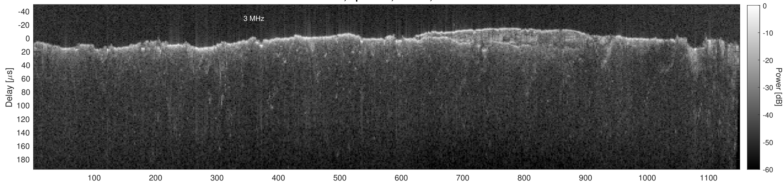
Orbit 15149, Cluttergram
