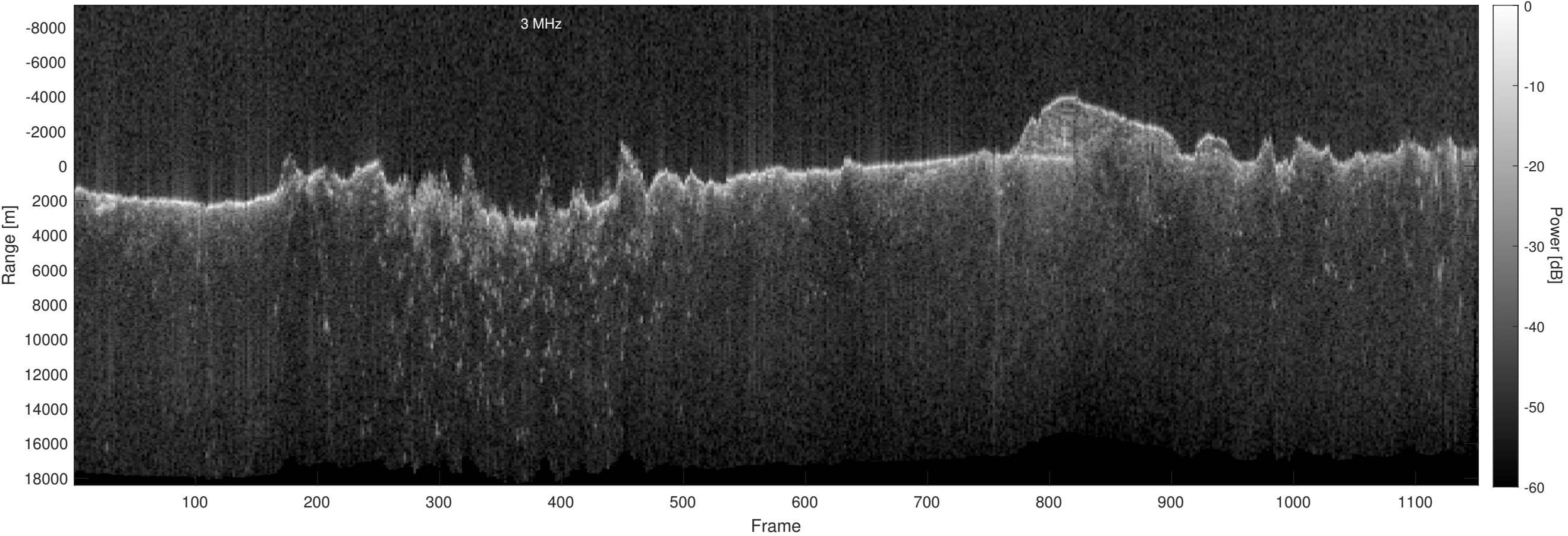
Orbit 15151, Optimized, Window, Depth-Corrected, Channel 2
