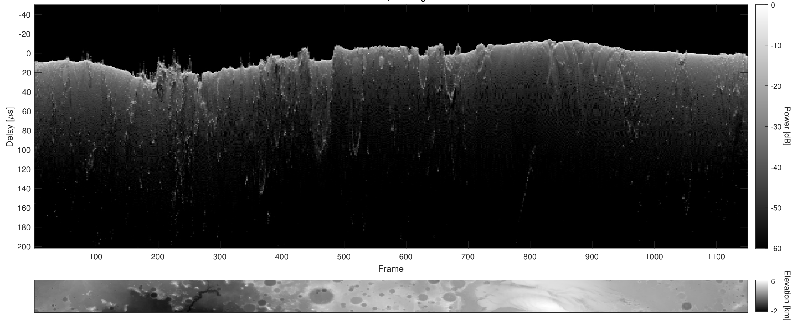
Orbit 15153, Cluttergram
