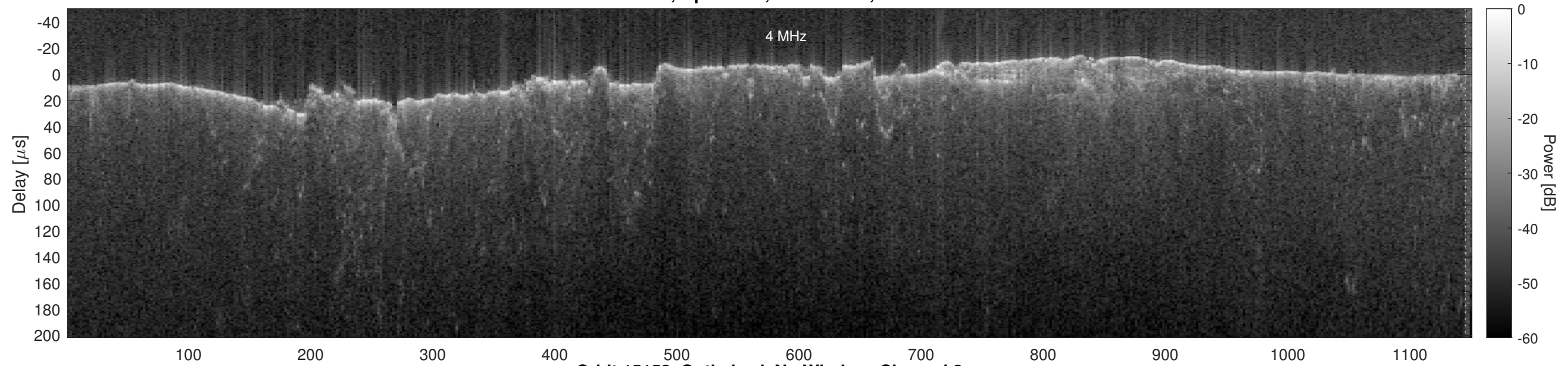
Orbit 15153, Optimized, No Window, Channel 2
