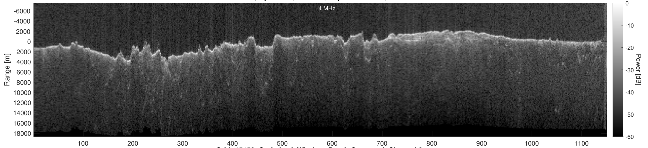
Orbit 15153, Optimized, Window, Depth-Corrected, Channel 2
