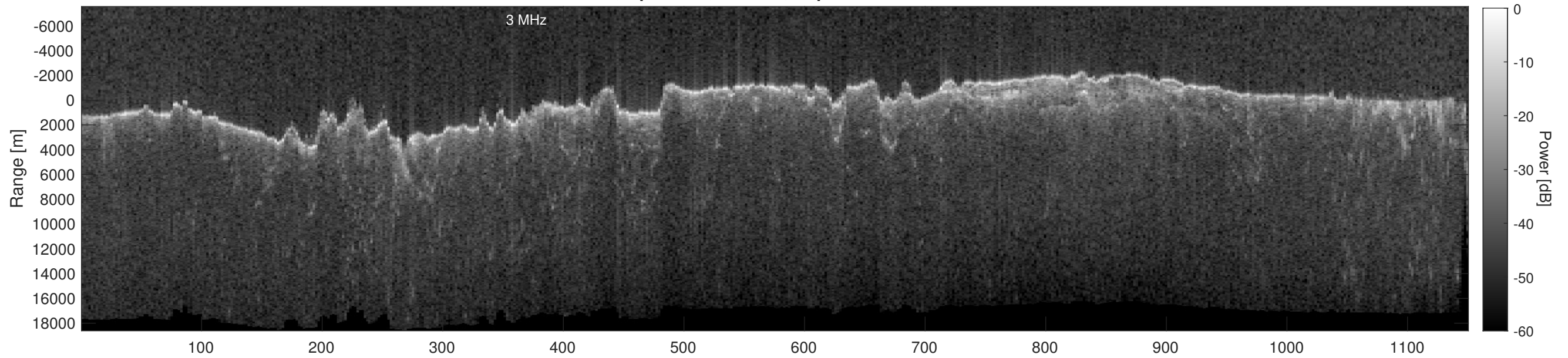
Orbit 15153, Depth-Corrected Cluttergram
