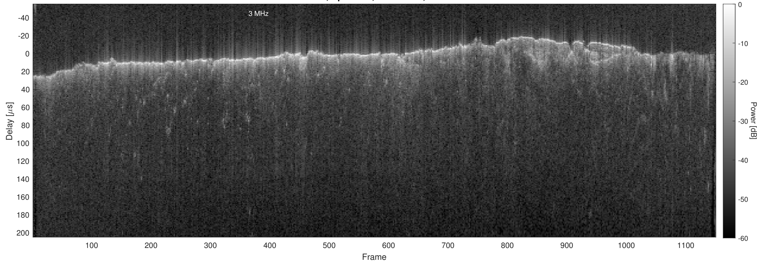
Orbit 15154, Optimized, No Window, Channel 2
