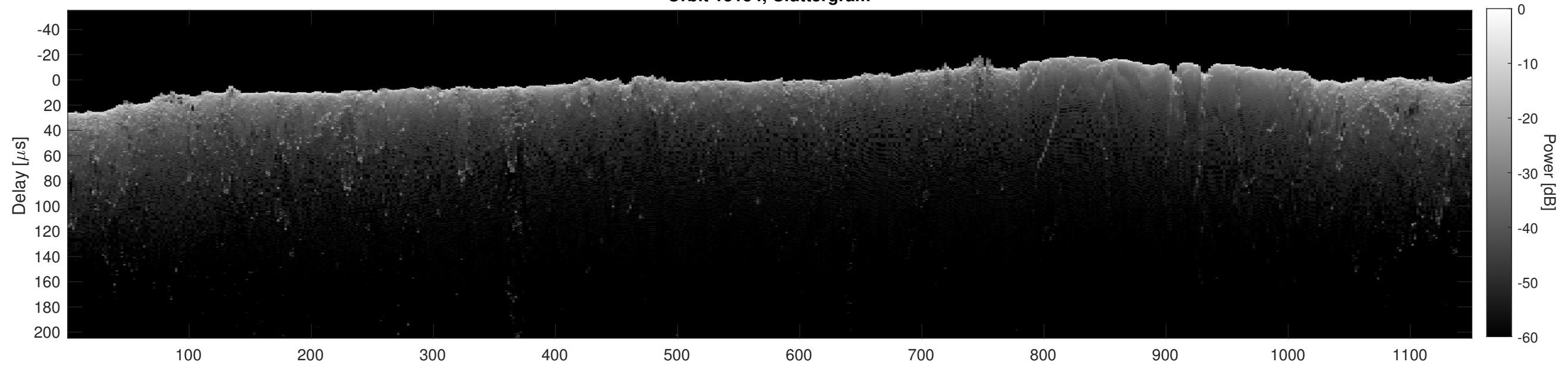
Orbit 15154, Cluttergram
