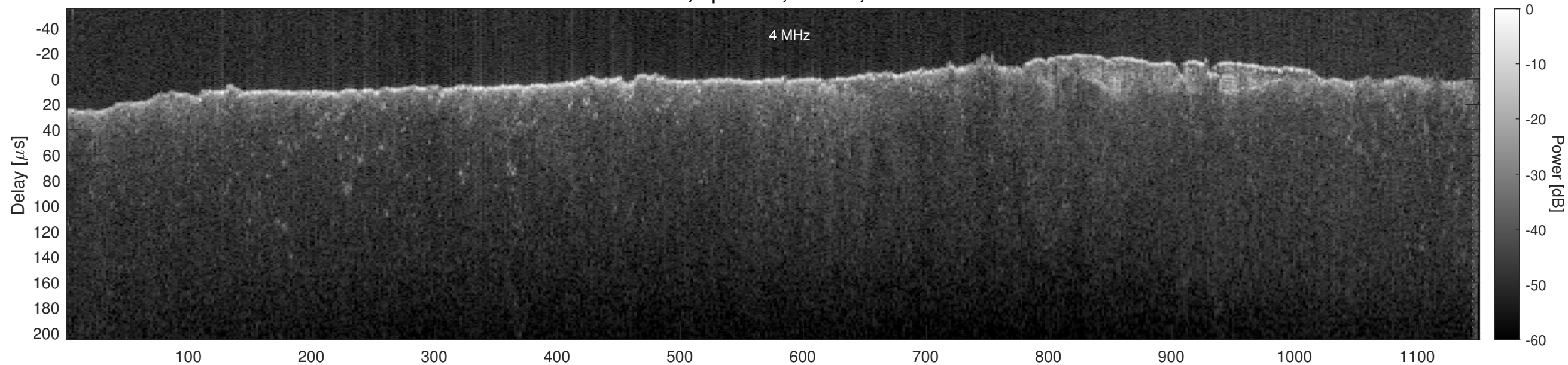
Orbit 15154, Optimized, Window, Channel 2
