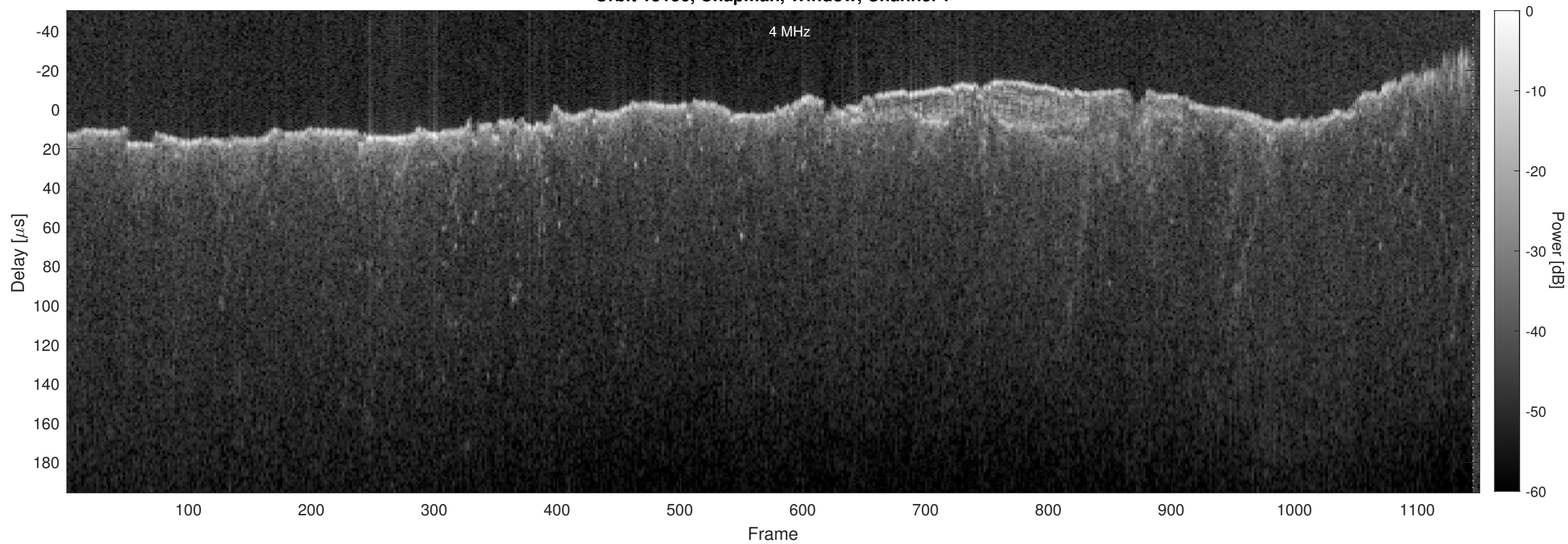
Orbit 15156, Chapman, Window, Channel 2
