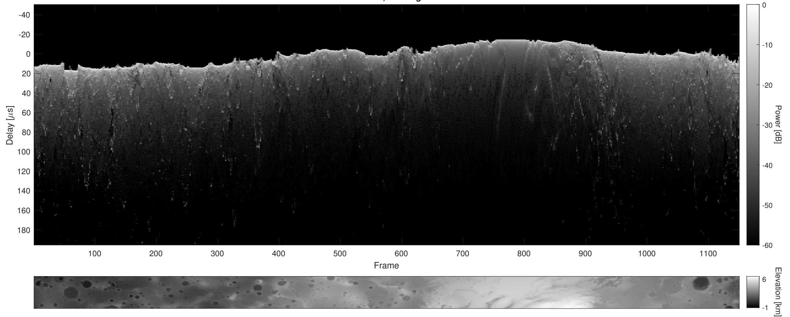
Orbit 15156, Cluttergram
