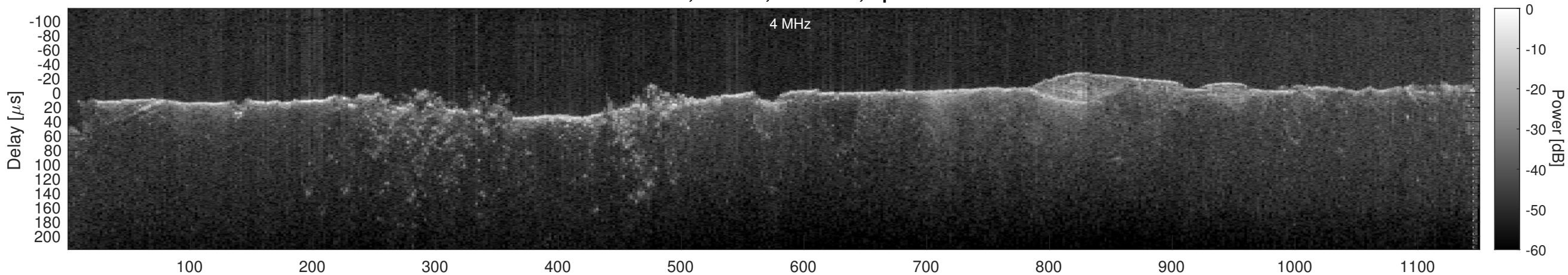
Orbit 15158, Cluttergram
