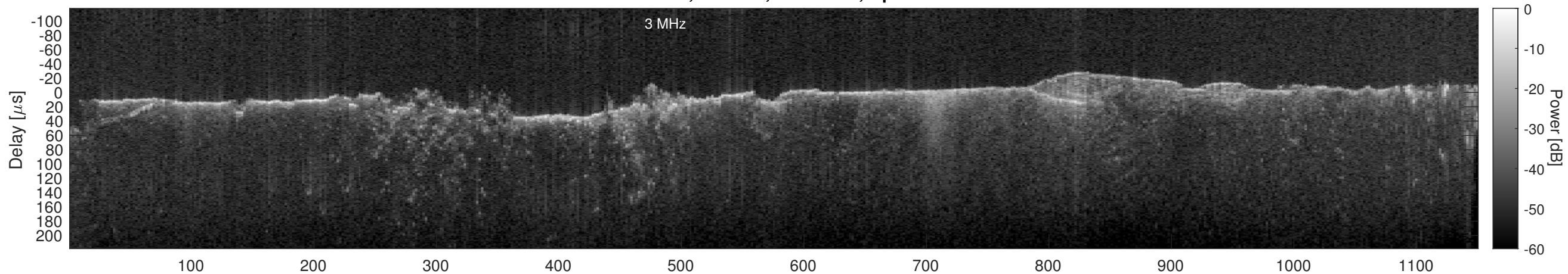
Orbit 15158, Cluttergram
