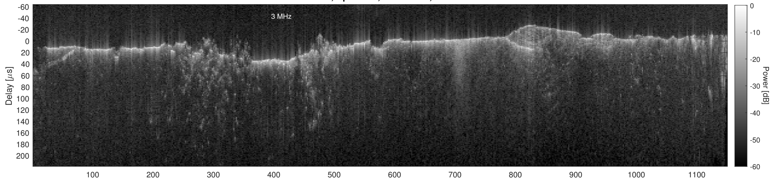
Orbit 15158, Cluttergram
