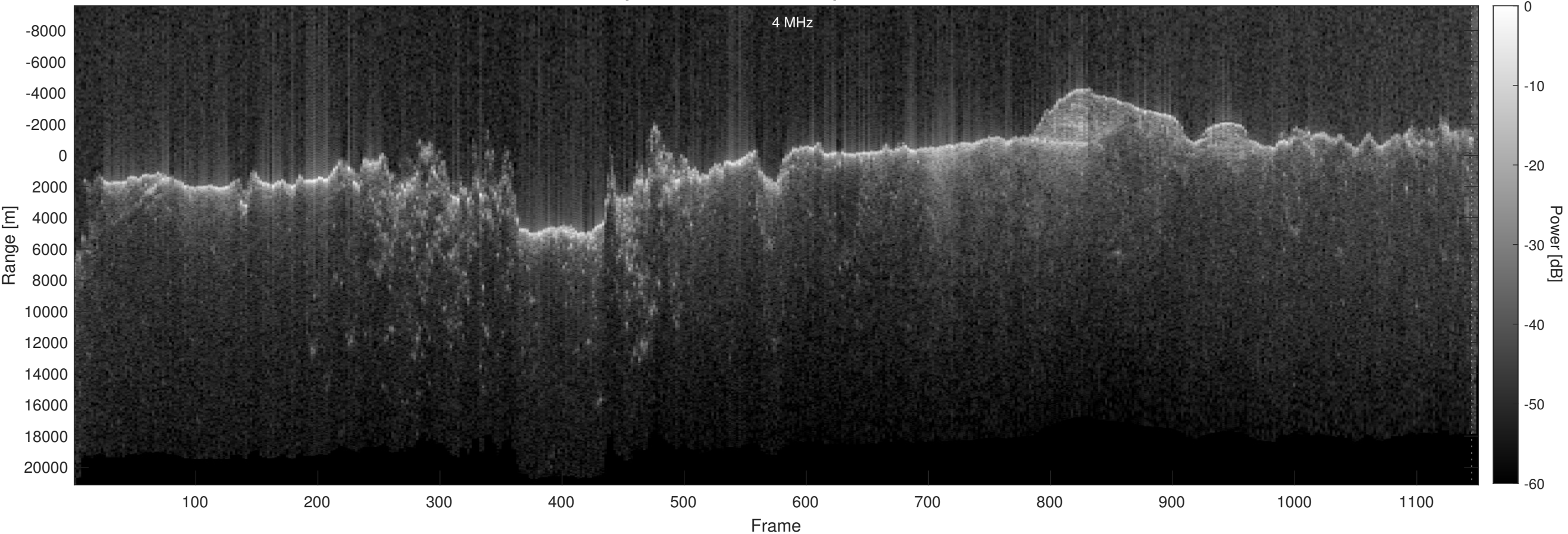
Orbit 15158, Optimized, No Window, Depth-Corrected, Channel 2
