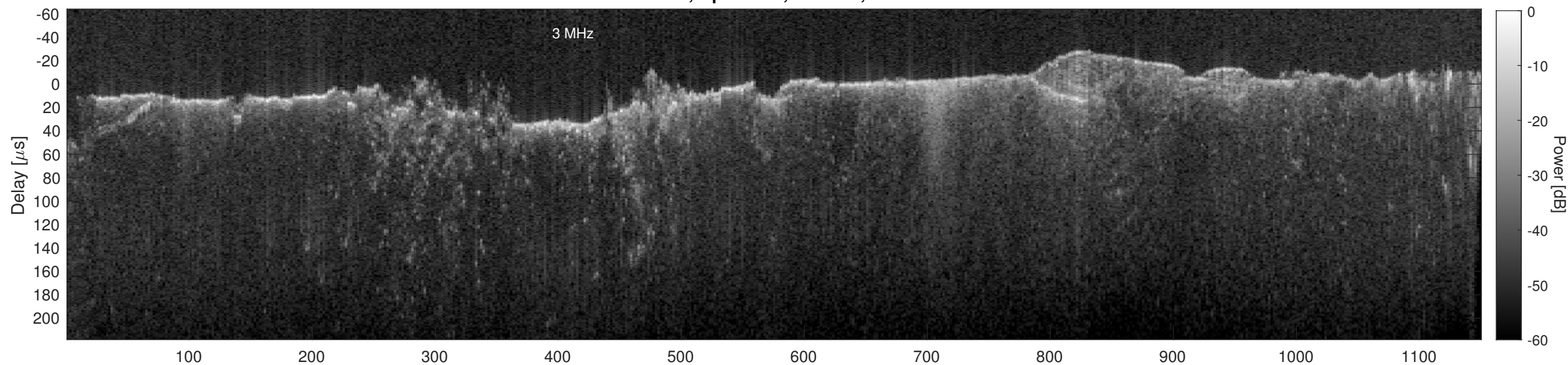
Orbit 15158, Cluttergram
