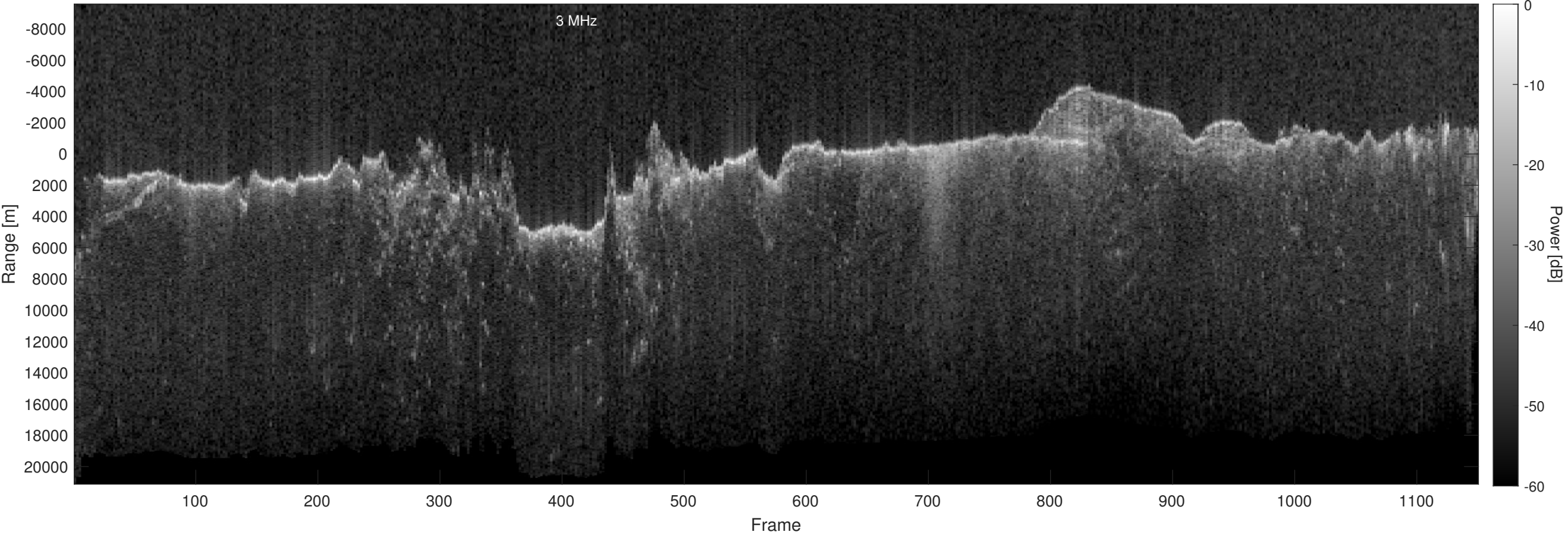
Orbit 15158, Optimized, Window, Depth-Corrected, Channel 2
