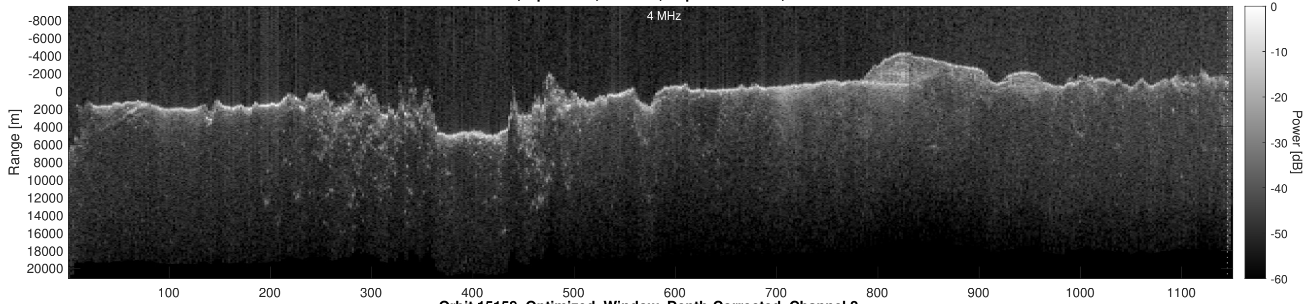
Orbit 15158, Optimized, Window, Depth-Corrected, Channel 2
