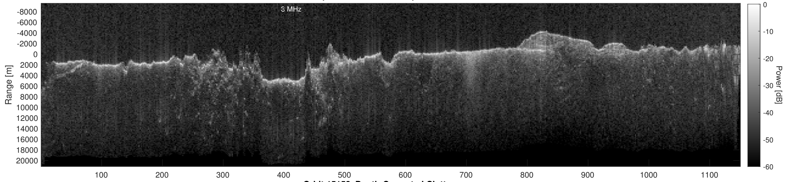
Orbit 15158, Depth-Corrected Cluttergram
