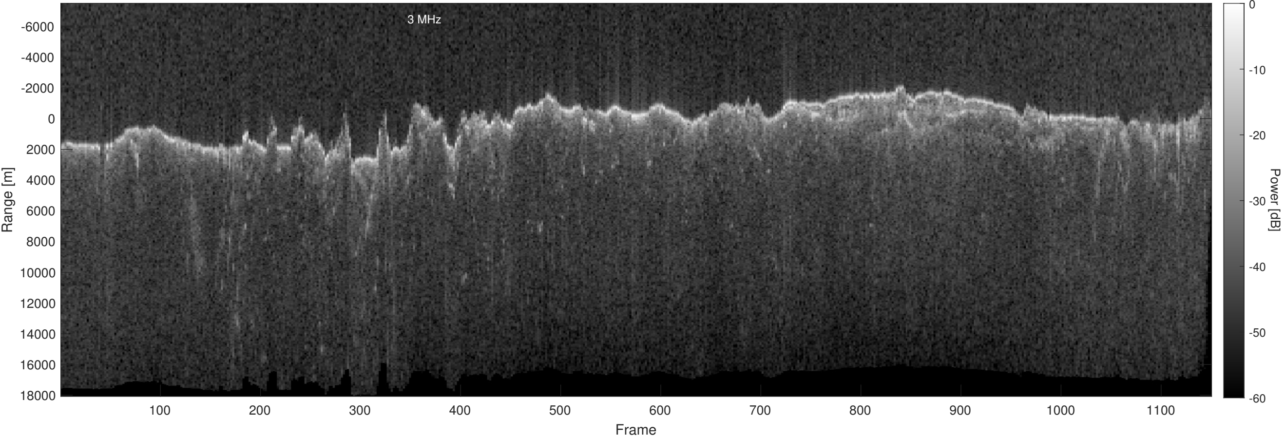
Orbit 15160, Optimized, Window, Depth-Corrected, Channel 2
