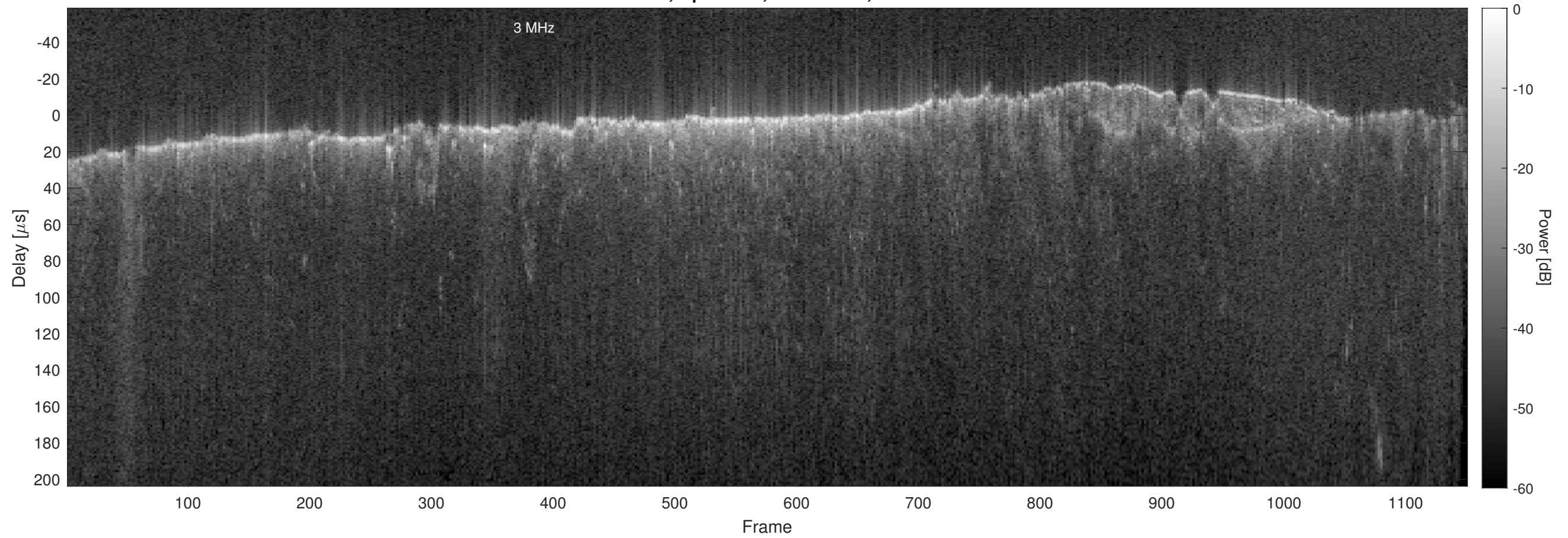
Orbit 15161, Optimized, No Window, Channel 2
