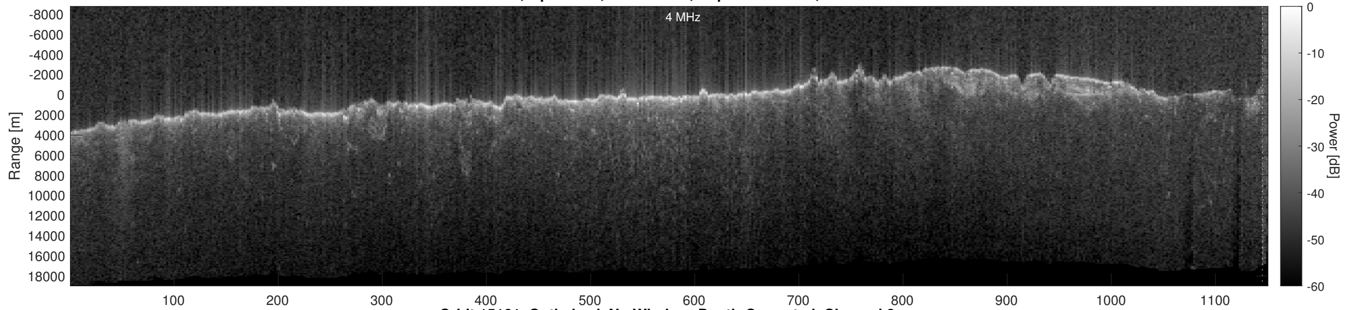
Orbit 15161, Optimized, No Window, Depth-Corrected, Channel 2
