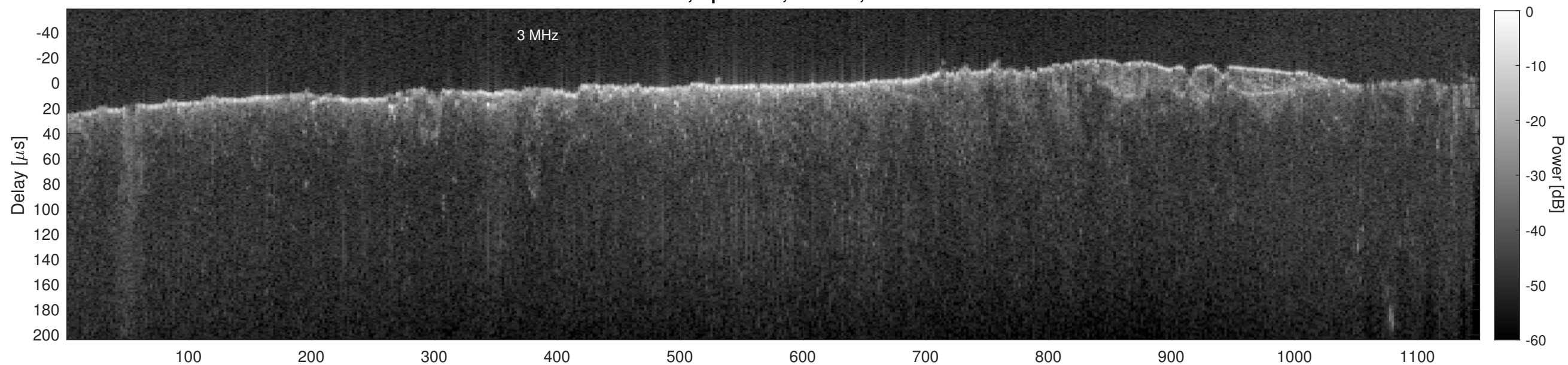
Orbit 15161, Cluttergram
