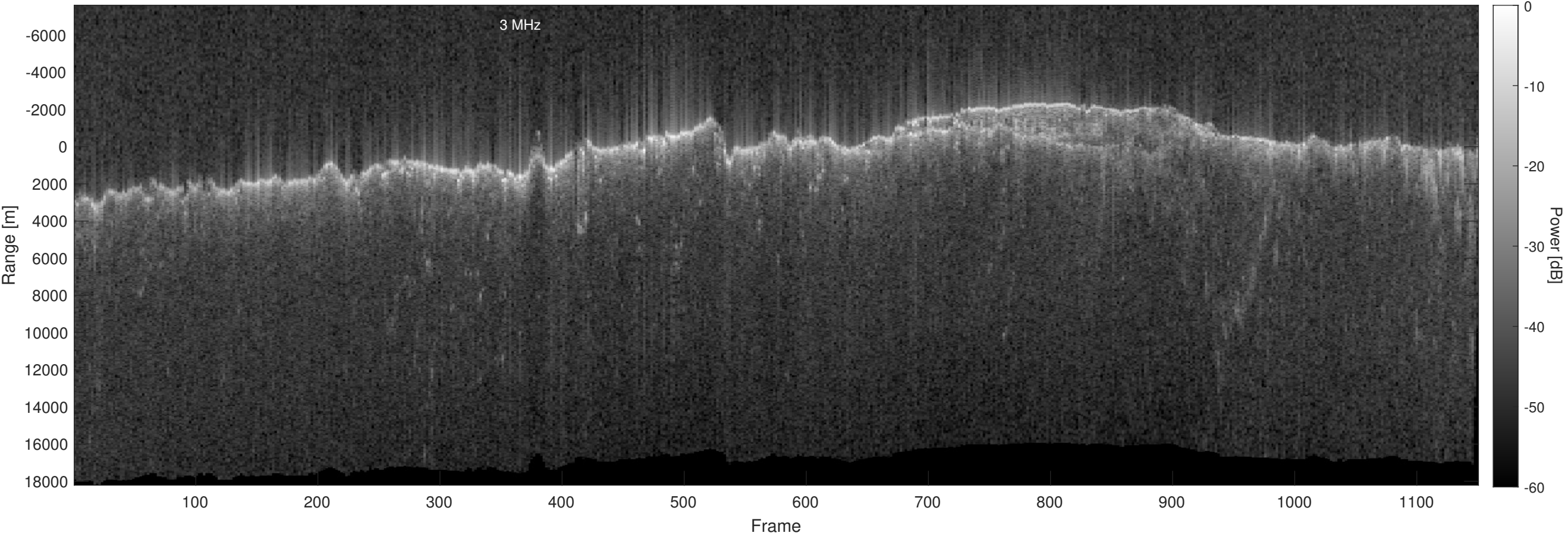
Orbit 15163, Optimized, No Window, Depth-Corrected, Channel 2
