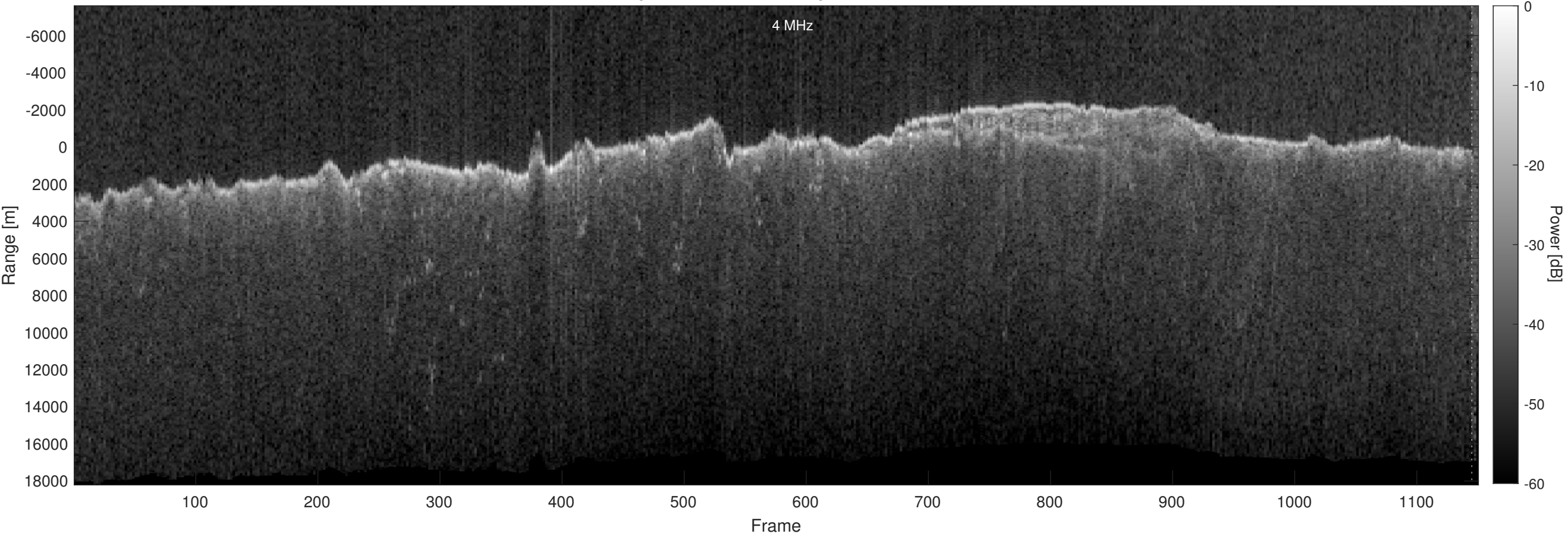
Orbit 15163, Optimized, Window, Depth-Corrected, Channel 2
