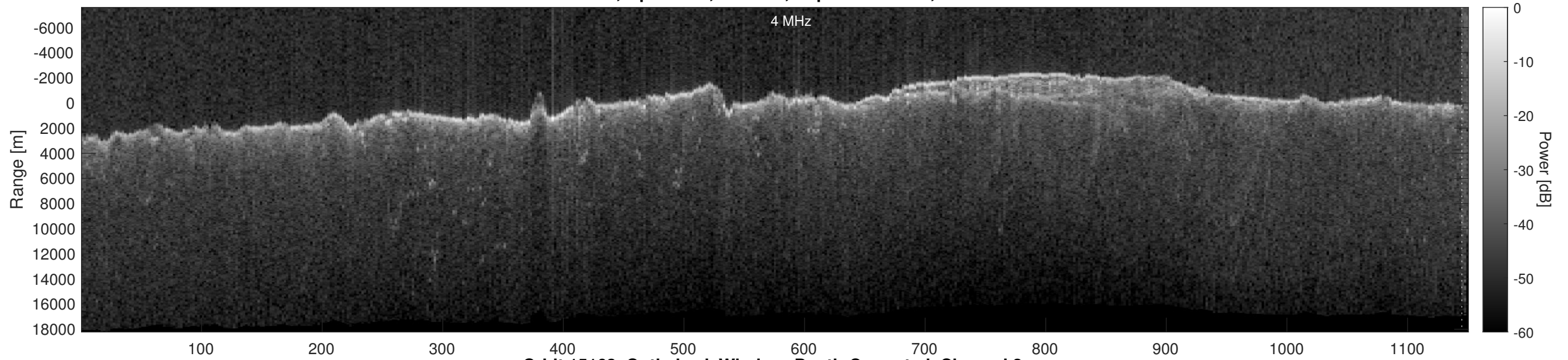
Orbit 15163, Optimized, Window, Depth-Corrected, Channel 2
