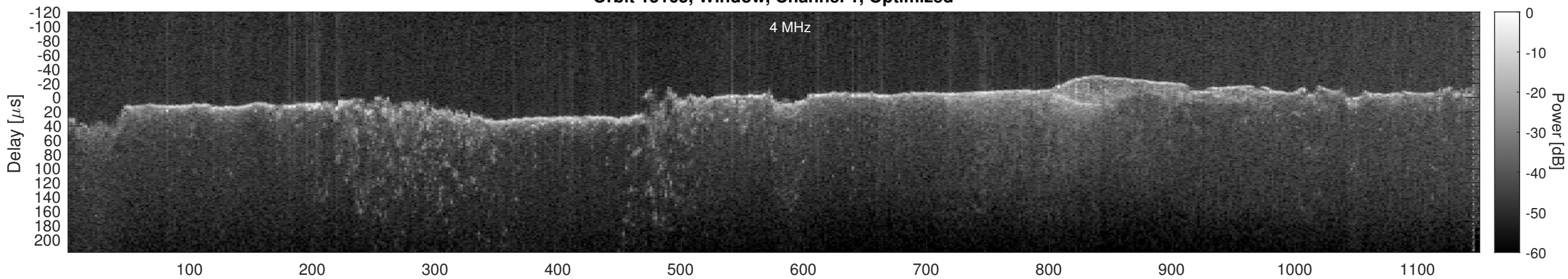
Orbit 15165, Cluttergram
